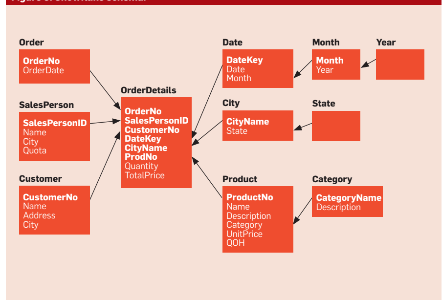
Figure 3. Snowflake schema.
